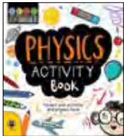
Physics Activity Book 9781911509202 PB £6.99 Feb 18
